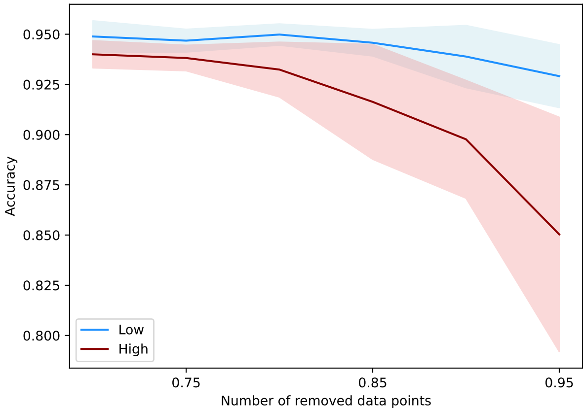
DataAttrOpt(5000, 0.03, 15, best, alpha=best) - bbc-embeddings
